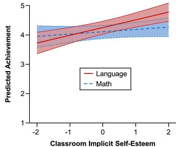
FIGURE 3 Model-predicted relations between type of achievement and classroom-level implicit self-esteem by grade level. Model-predicted relations between classroom-level implicit self-esteem and language (red) and math (blue) achievement for Grade 1 and Grade 5 shown. Shaded regions indicate 95% confidence intervals. The implicit self-esteem–language achievement relation was significant for Grade 5 ( p = .050 ); no other slopes were significant ( ps > .05 ).
